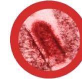
Lyssavirus
